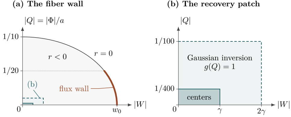
Figure 1: The fixed fiber in modulus coordinates. The wave flux through r = 0 is supported on the heavy arc, where |Q| \leq 1/20 and hence |W| \geq \sqrt{3} w_0/2 . This separation gives Gaussian decay e^{-cs/h} even for |v| \leq w_0/3 . In the enlargement (b), once K\gamma is large, the radius- h balls about the marked centers project into the dashed patch. There |W - v| \leq 4\gamma on the enlarged cap |v| \leq 2\gamma , so Gaussian inversion costs at most e^{C\gamma^2 s/h} . The aperture \gamma is fixed independently of h ; its size relative to w_0 is schematic.
