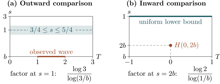
Figure 2: The two comparisons, with radii s = |\tau| drawn schematically. The boundary mass on 1 \leq T \leq 2 bounds the mass in the shaded band from below. The mean inequality on a fixed annulus supplies a lower bound on the entire upper wall in (b). The two displayed fractions are values of the normalized radial harmonic functions. The comparison solutions with potential dominate fixed multiples of these values, giving the factor [\log(3/b)]^{-2} at the dot. In the wave estimate, b = 2Kh : H controls the wave norm on the marked segment and is controlled by the initial data at the dot.
